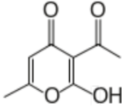
1. Dehydroacetic acid(DA)
